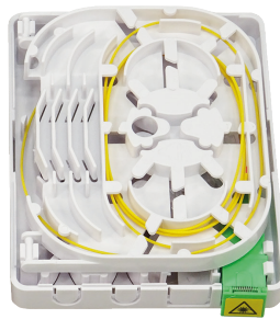
FTB-3200-KSA
